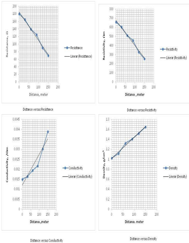
Fig.5. Resistance, Resistivity, Conductivity and Density
