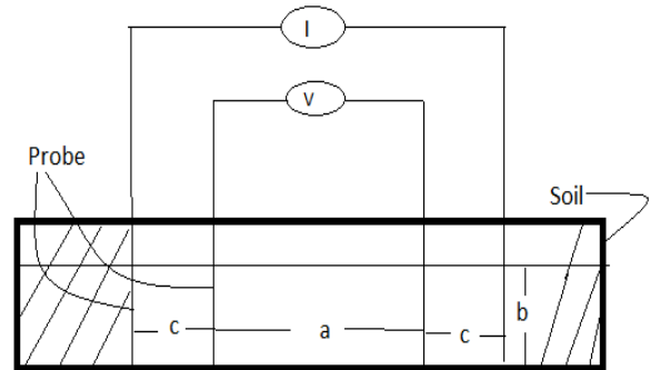
Fig.4. Measurement Technique
